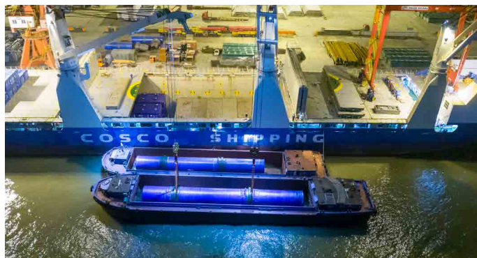
Drum 32m 140 tons to Malaysia
